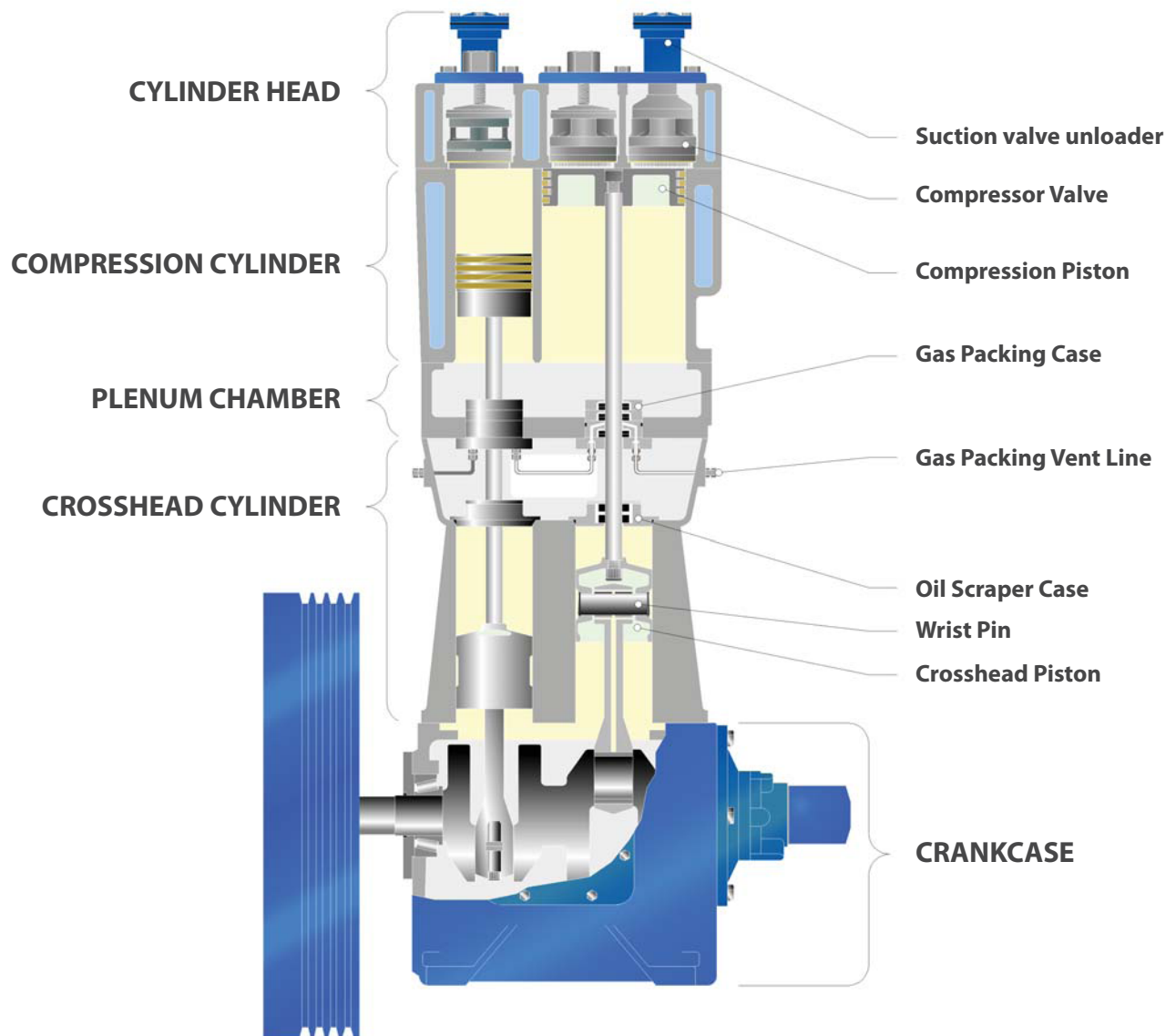
Model 2WN61 Gas Compressor
